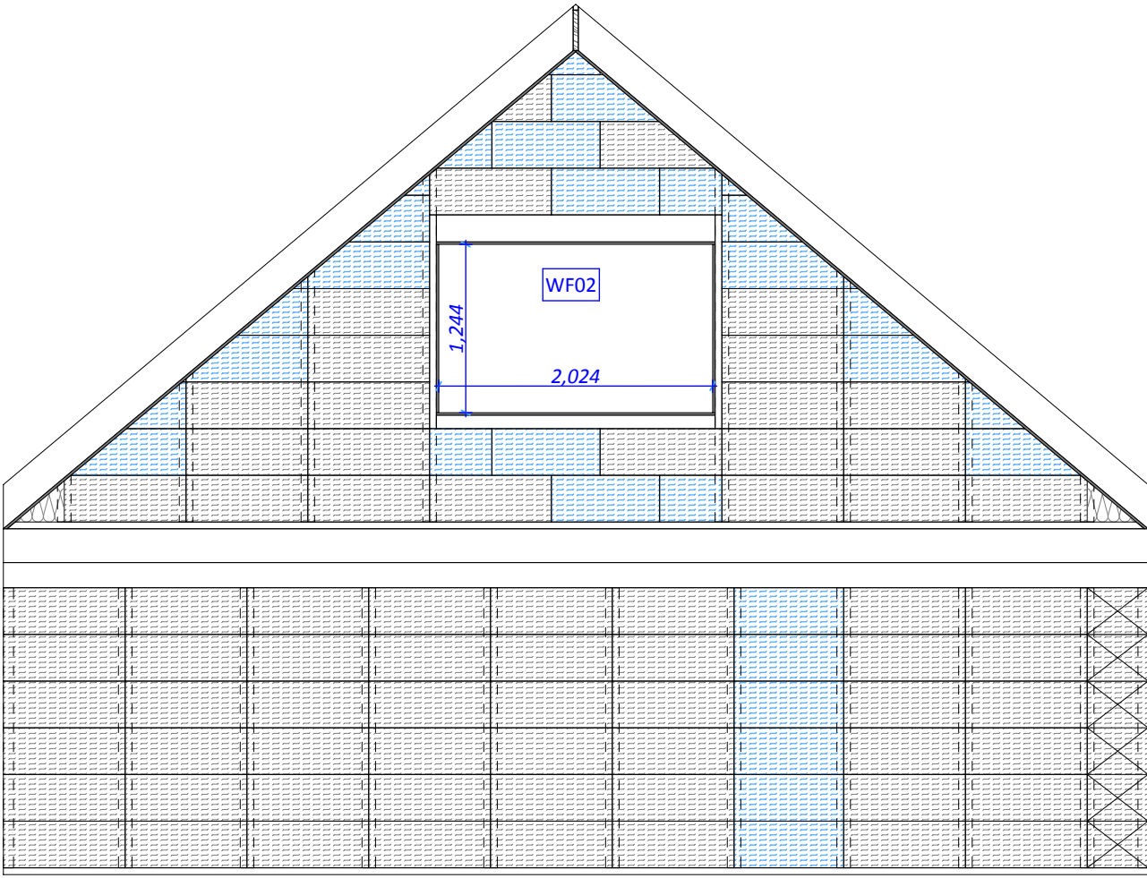
East Bale Elevation
