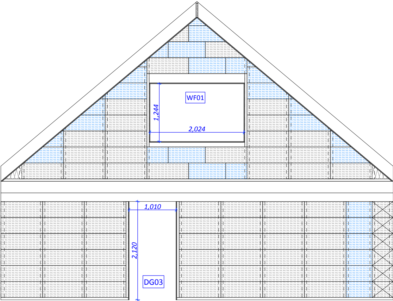
West Bale Elevation
